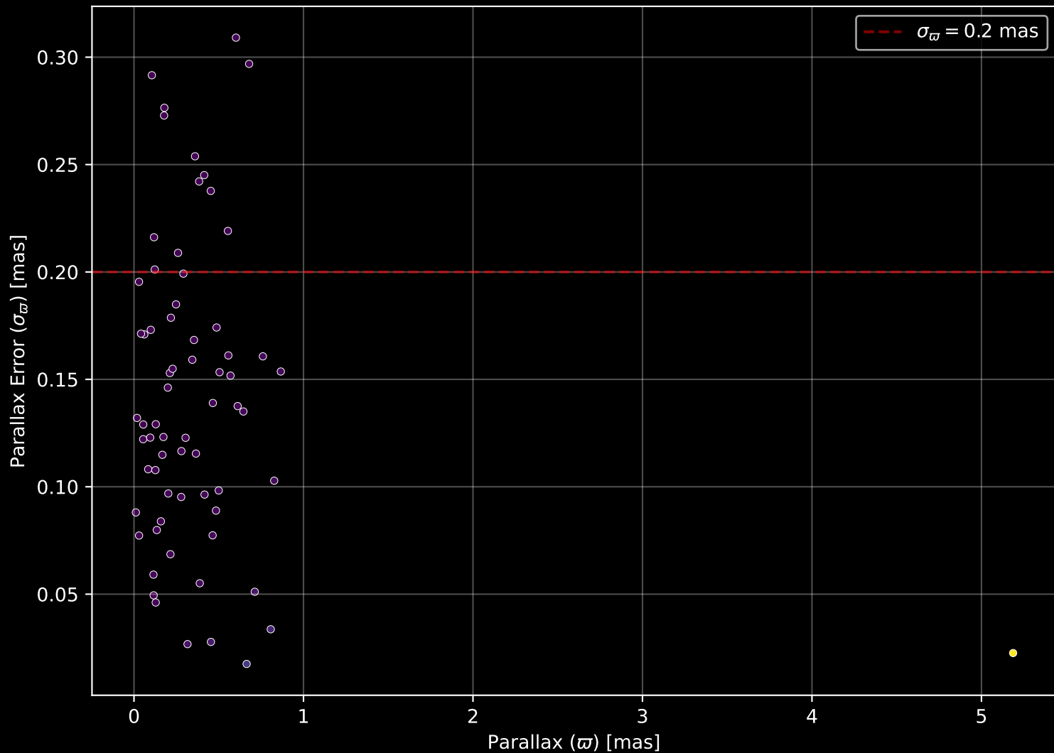
APOGEE DR17 Field: [000-02-O] Parallax Quality (n= 68)
