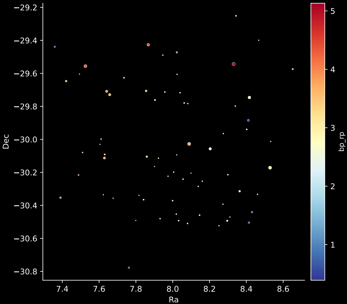
APOGEE DR17 Field: [000-02-O] Stars: 68
