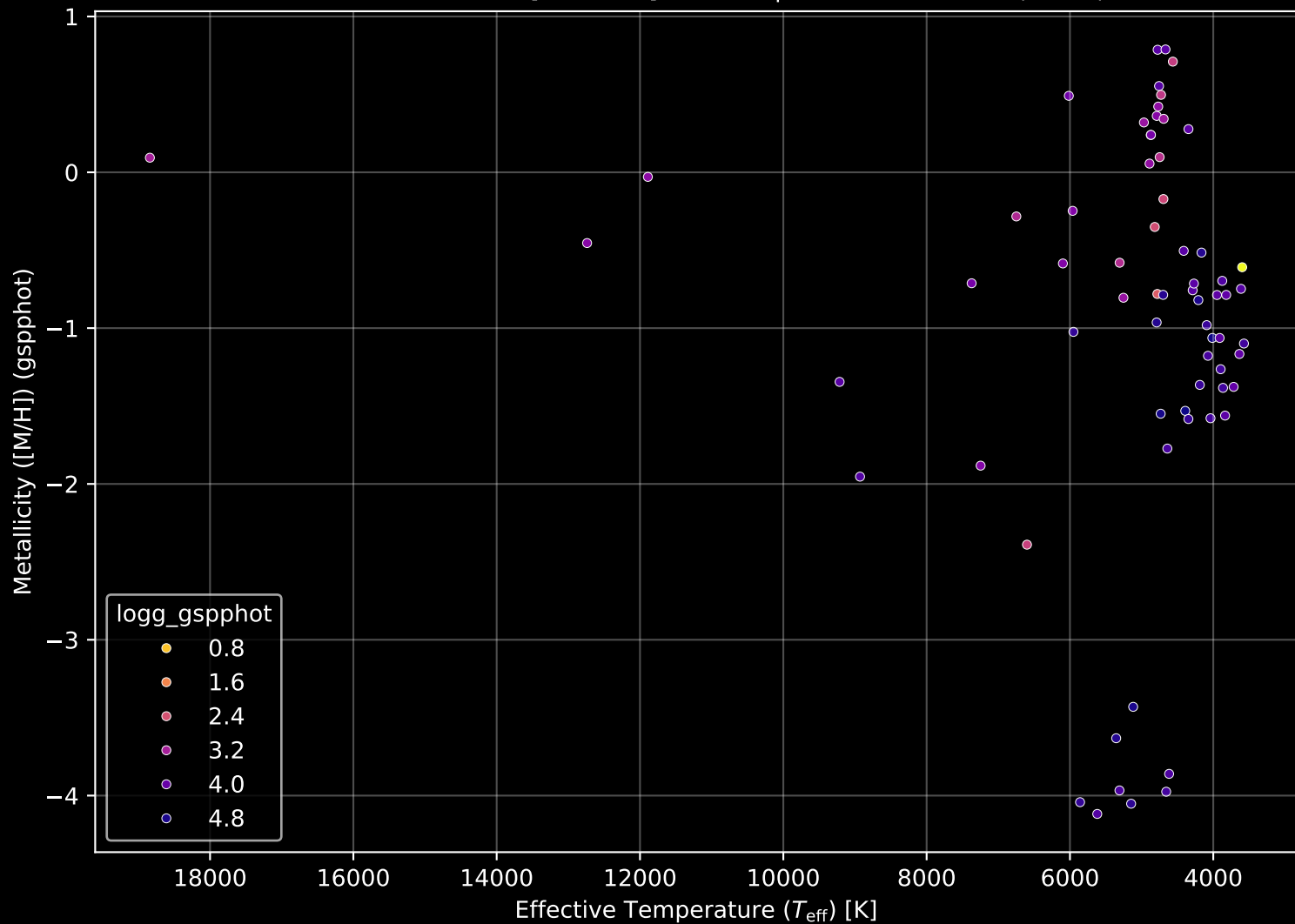
APOGEE DR17 Field: [000-02-O] Stellar Population Parameters (n= 68)
