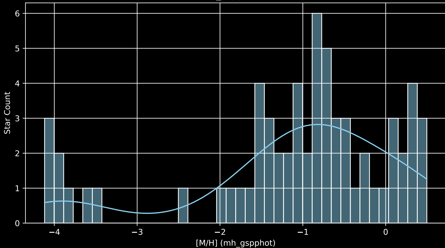
APOGEE DR17 Field: [000-02-O [M/H] (mh_gspphot) (n= 64)
