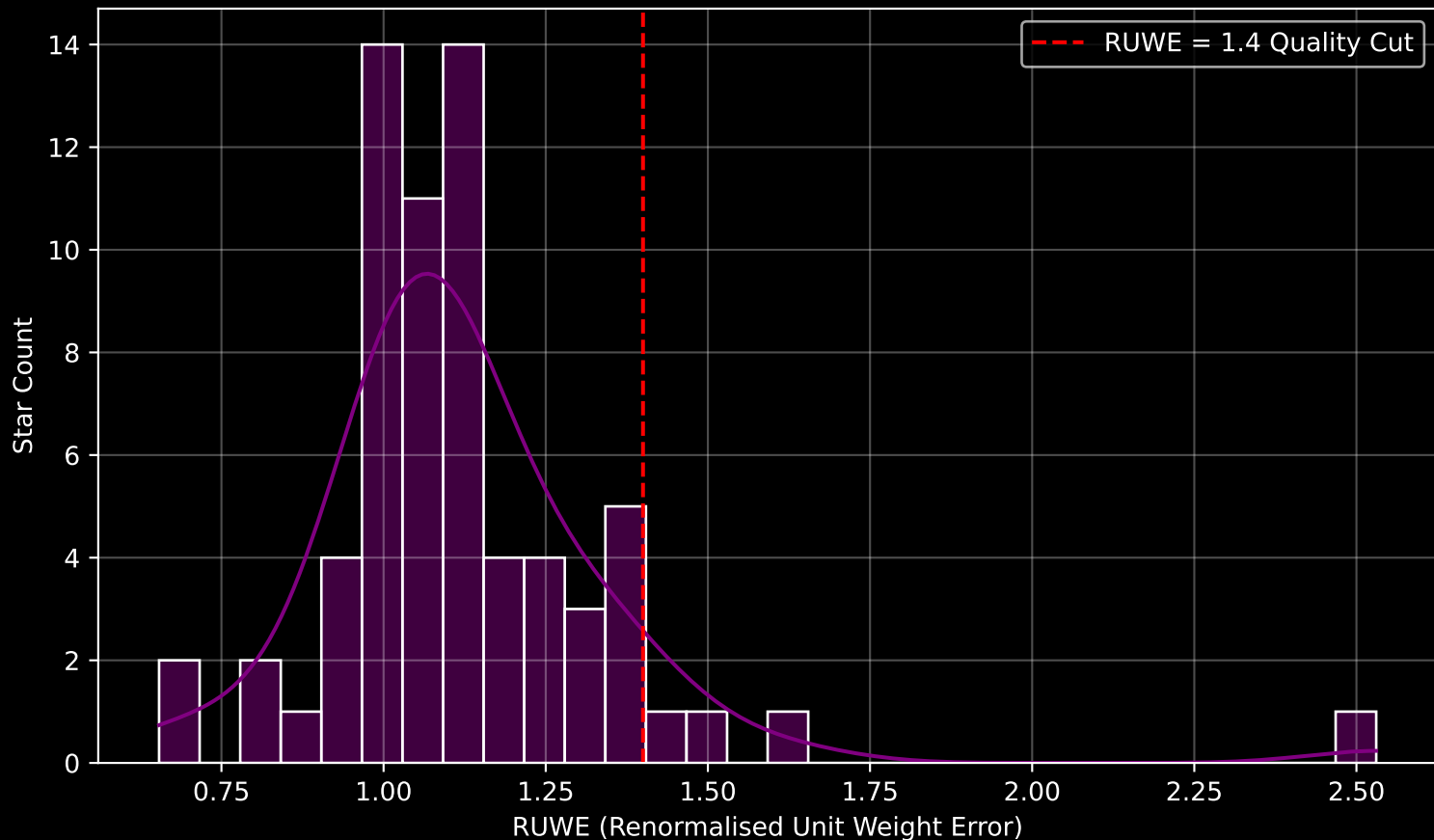
GAPOGEE DR17 Field [000-02-O] RUWE Distribution (n= 68)
