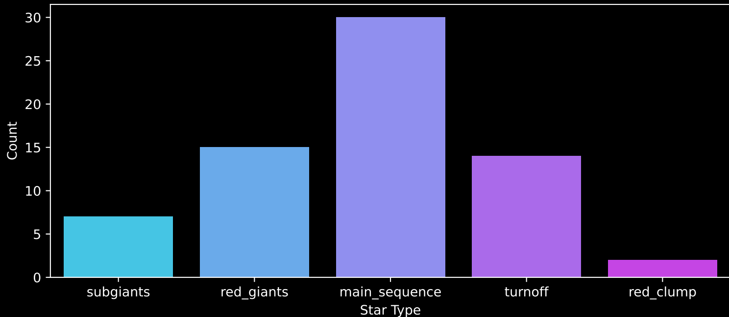
APOGEE DR17 Field: [000-02-O] Count plot of Star Type
