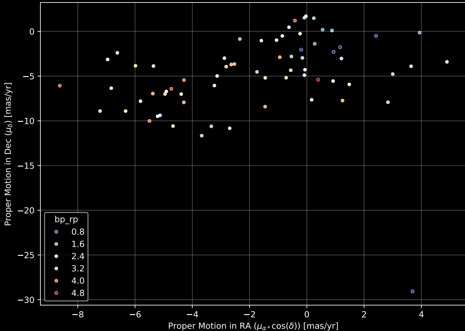
APOGEE DR17 Field: [000-02-O] Proper Motion Diagram (n= 68)
